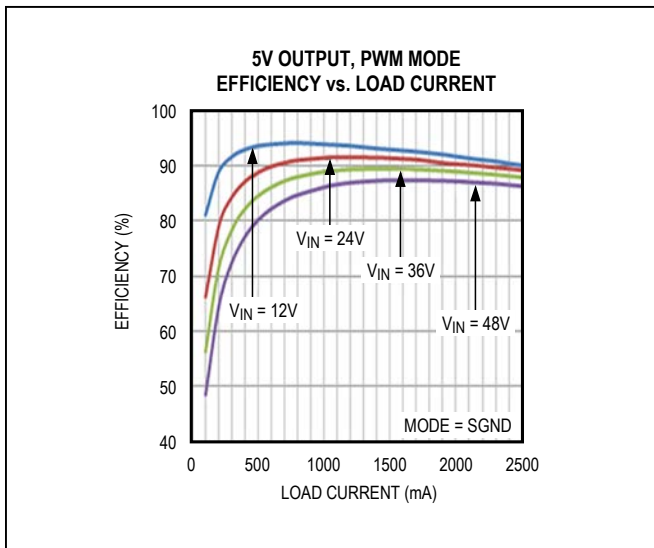
Figure 2. MAX17503 5V Output Efficiency (PWM Mode)
