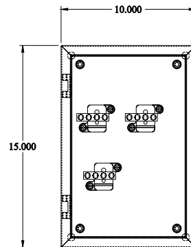
FRONT VIEW - COVER REMOVED
