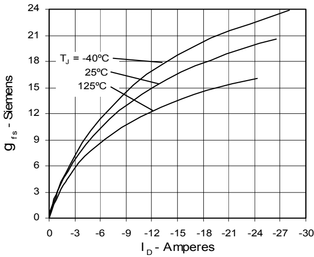
Fig. 7. Transconductance
