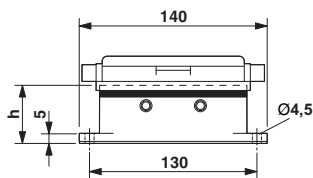
Dimensional drawing
