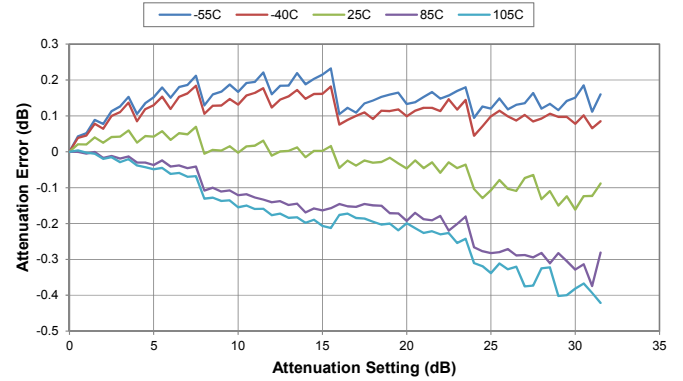
Figure 20. Attenuation Error @ 100 MHz vs Temperature
