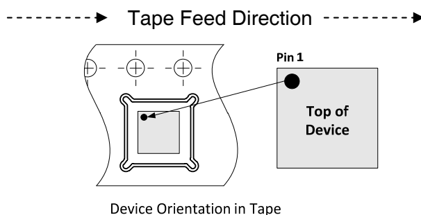
Device Orientation in Tape
