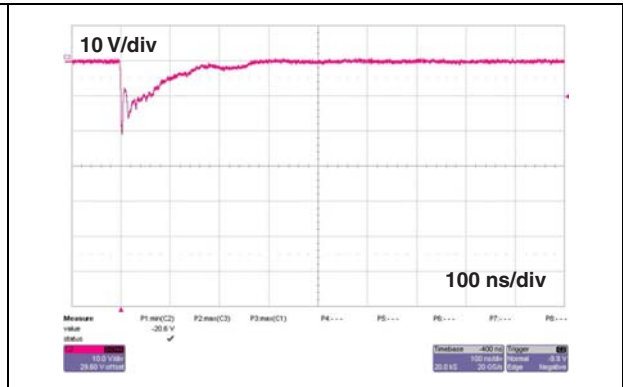
Figure 9. Remaining voltage on V_{BUS} after USBULC-2P6 during negative ESD surge (-15 kV air discharge)
