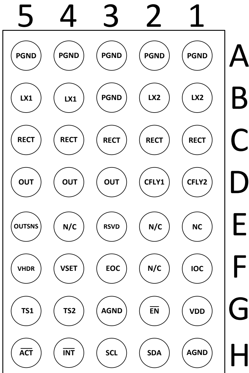
Bottom View
