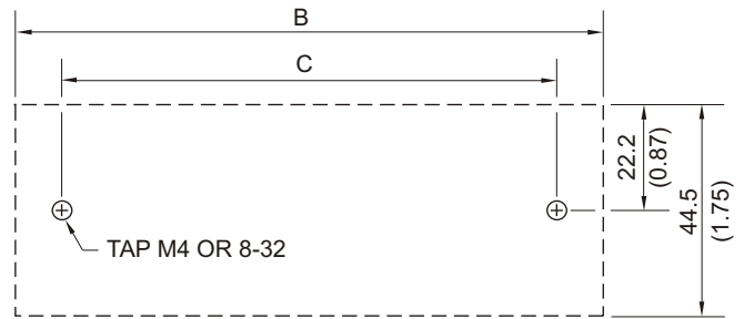
MOUNTING DETAIL
