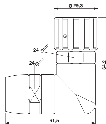
Dimensioned drawing
