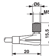
Dimensioned drawing
