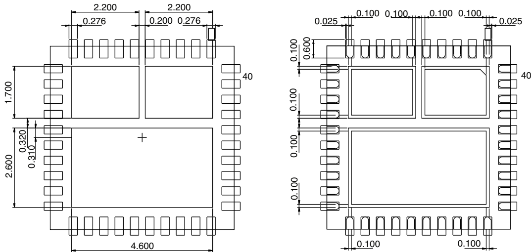
Figure 9 - PowerPAK MLP 66-40
