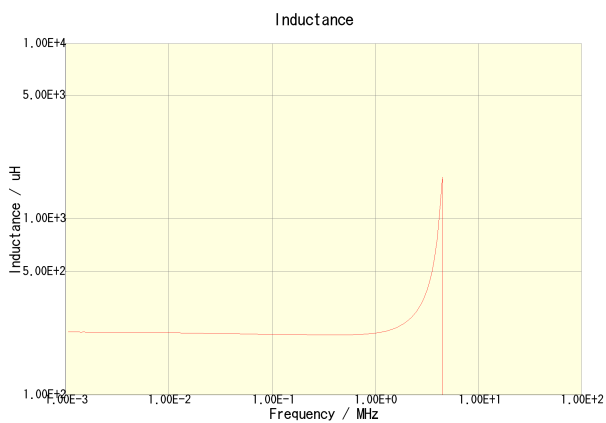
CLF7045T-221M-CA
