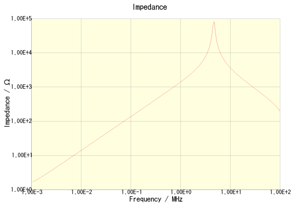
CLF7045T-221M-CA
