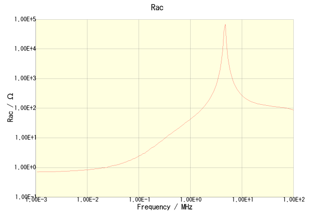
CLF7045T-221M-CA
