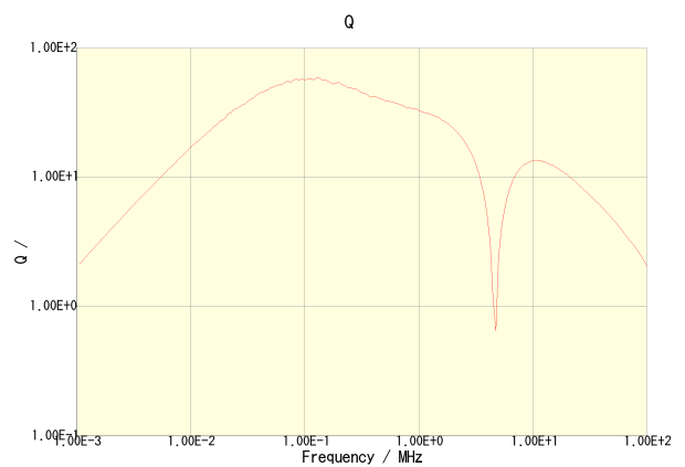
CLF7045T-221M-CA
