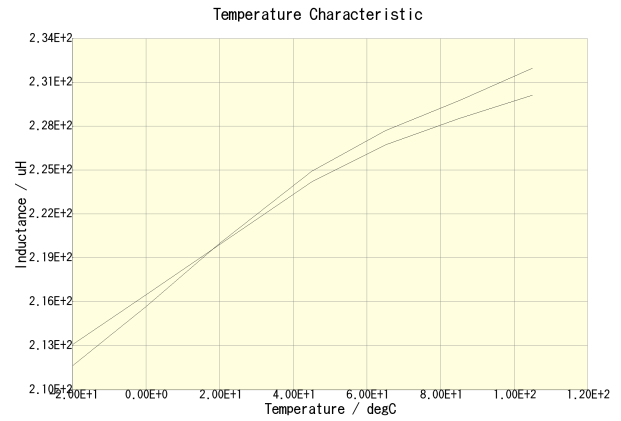
CLF7045T-221M-CA(DC = 0A)
