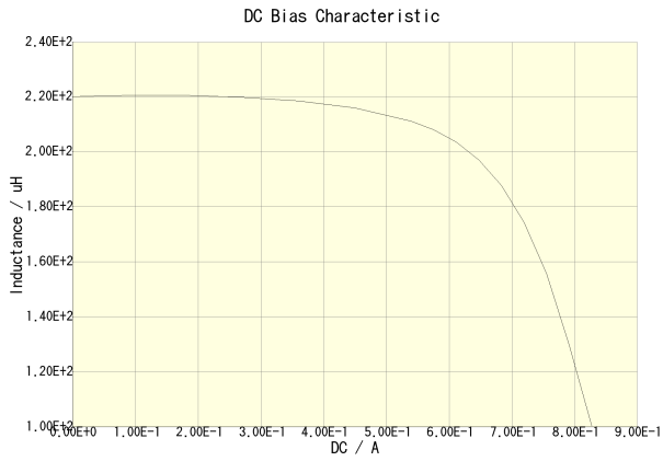
CLF7045T-221M-CA(Amb. Temp. = 20degc)
