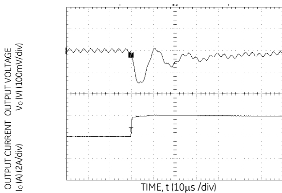
Figure 15. Transient Response to Dynamic Load change from 50% to 100% of full load with di/dt of 5A/µs.
