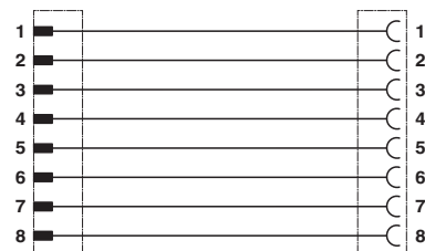
Contact assignment of the M12 connector and the M12 socket
