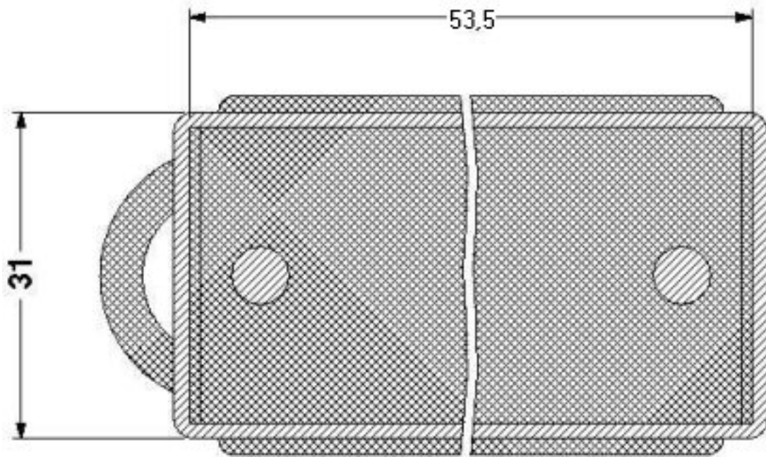
Dimensioned drawing
