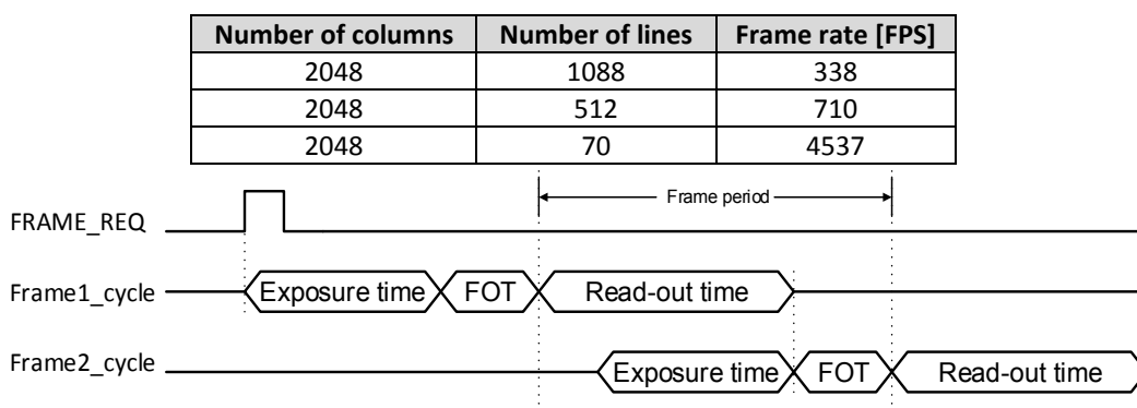
FIGURE 6: FRAME PERIOD
