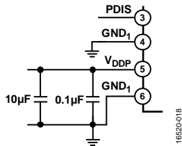
Figure 21. ADuM5020 V_{DDP} Bias and Bypass Components
