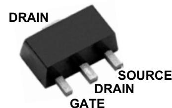
TO-243AA (SOT-89)
