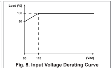
Fig. 5. Input Voltage Derating Curve
