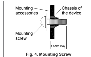
Fig. 4. Mounting Screw
