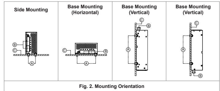
Fig. 2. Mounting Orientation
