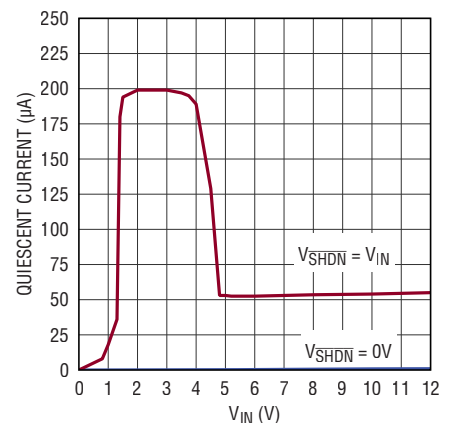
LT3061-5 Quiescent Current
