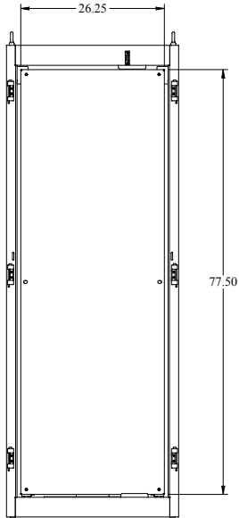
FRONT DOOR REMOVED
