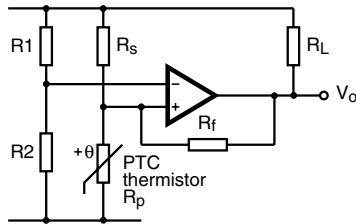
Fig. 1 Typical comparator circuit
