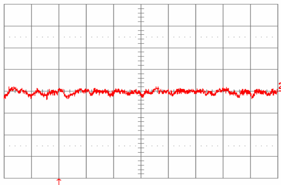
Fig. 25: Input reflected ripple current, i_s (10 mA/div), measured through 10 \mu\text{H} at the source at full rated load current and V_{in} = 48 \text{ V} . Refer to Fig. 23 for test setup. Time scale: 1\mu\text{s}/\text{div} .
