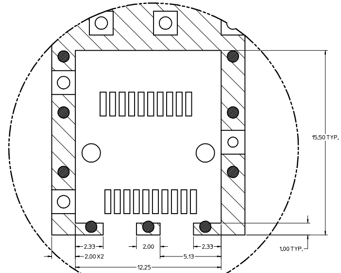
DETAIL1 SCALE 10:1 HOST CONNECTOR DETAIL
