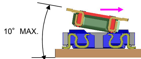
長手方向 "a" Direction (lengthways)
