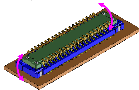
左右に少しずつ振りながら抜く（長手方向） Releasing the plug by moving slowly in "a" direction. (lengthways)
