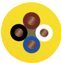
PVC yellow 105 °C [547]
