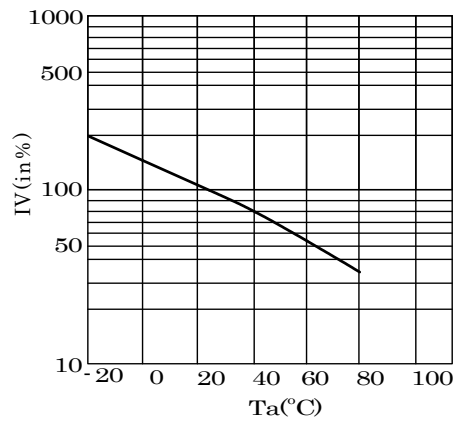
IV-Ta Characteristics
