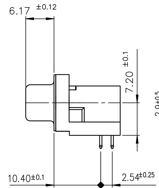
View shown without plastic pin
