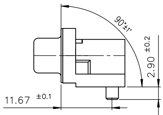
Detail of integral plastic pin
