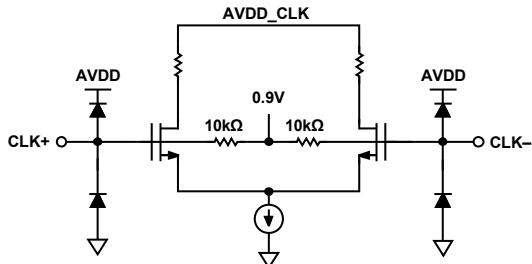
Figure 43. Equivalent Clock Circuit
