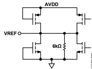
Figure 51. Equivalent VREF Circuit
