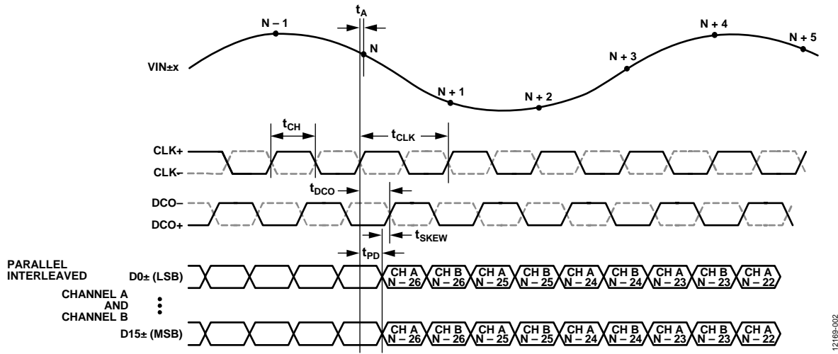
Figure 2. LVDS Data Output Timing
