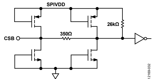
Figure 48. Equivalent CSB Input Circuit
