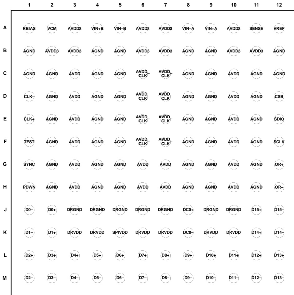
Figure 5. Pin Configuration
