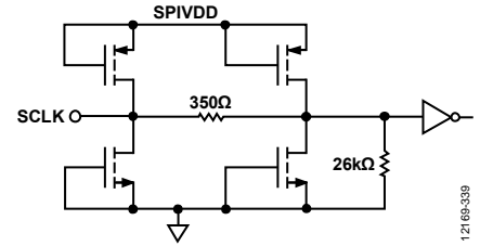
Figure 47. Equivalent SCLK Input Circuit
