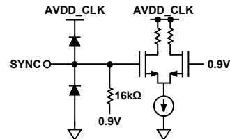
Figure 49. Equivalent SYNC Input Circuit
