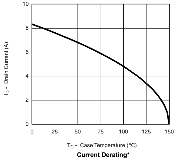
Current Derating*
