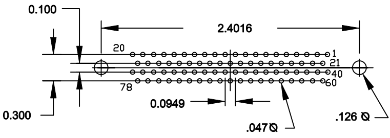
78 POSITION FEMALE
