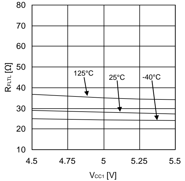
Figure 72. FLT Output ON-Resistance (IFLT=5mA)
