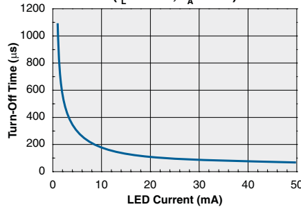
Typical Turn-Off Time vs. LED Forward Current ( I_L=60\text{mA} , T_A=25^\circ\text{C} )
