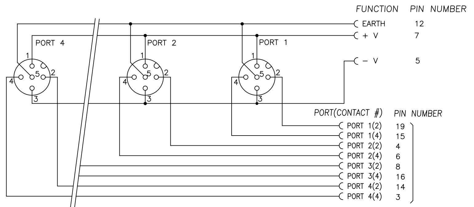
FACE VIEW OF END RECEPTACLE
