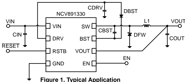
Figure 1. Typical Application
