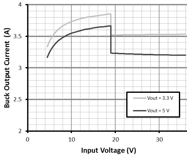
Figure 31. NCV891330 Load Current Capability with a 2.2 μH Inductor
