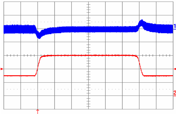
Fig. 19: Output voltage response to load current step-change (7.5 A – 15 A – 7.5 A) at V_{in} = 48\text{ V} . Top trace: output voltage (100 mV/div). Bottom trace: load current (5 A/div.). Current slew rate: 0.1 A/ \mu\text{s} . C_o = 1\ \mu\text{F} ceramic. Time scale: 0.2 ms/div.
