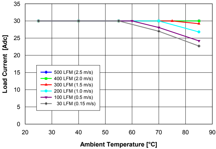
Fig. 9: Available load current vs. ambient air temperature and airflow rates for converter mounted vertically with V_{in} = 54\text{ V} , air flowing from pin 3 to pin 1 and maximum FET temperature \leq 120^{\circ}\text{C} .
