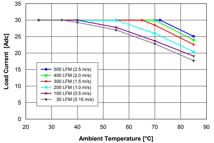
Fig. 10: Available load current vs. ambient air temperature and airflow rates for converter mounted vertically with V_{in} = 54\text{ V} , air flowing from pin 3 to pin 1 and maximum FET temperature \leq 105^{\circ}\text{C} .
