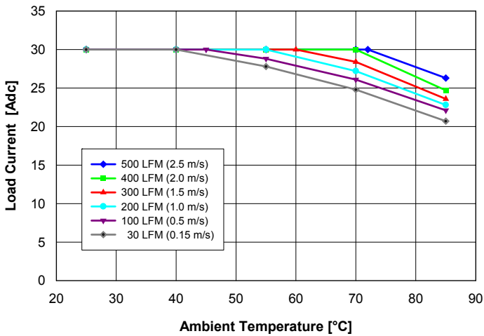
Fig. 11: Available load current vs. ambient temperature and airflow rates for converter mounted horizontally with V_{in} = 54\text{ V} , air flowing from pin 3 to pin 4 and maximum FET temperature \leq 120^{\circ}\text{C} .
