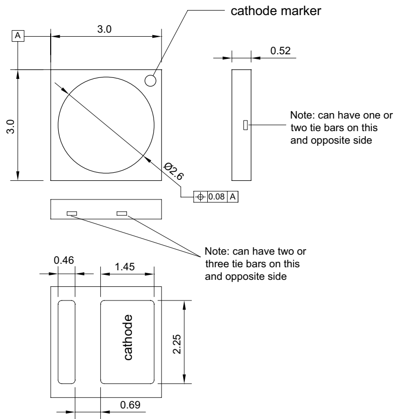
Figure 9. Mechanical dimensions for LUXEON 3030 2D.
