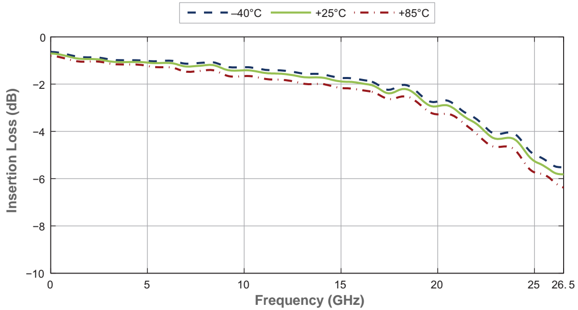
Figure 6 • Insertion Loss vs Temperature (RFC–RFX) (*)
