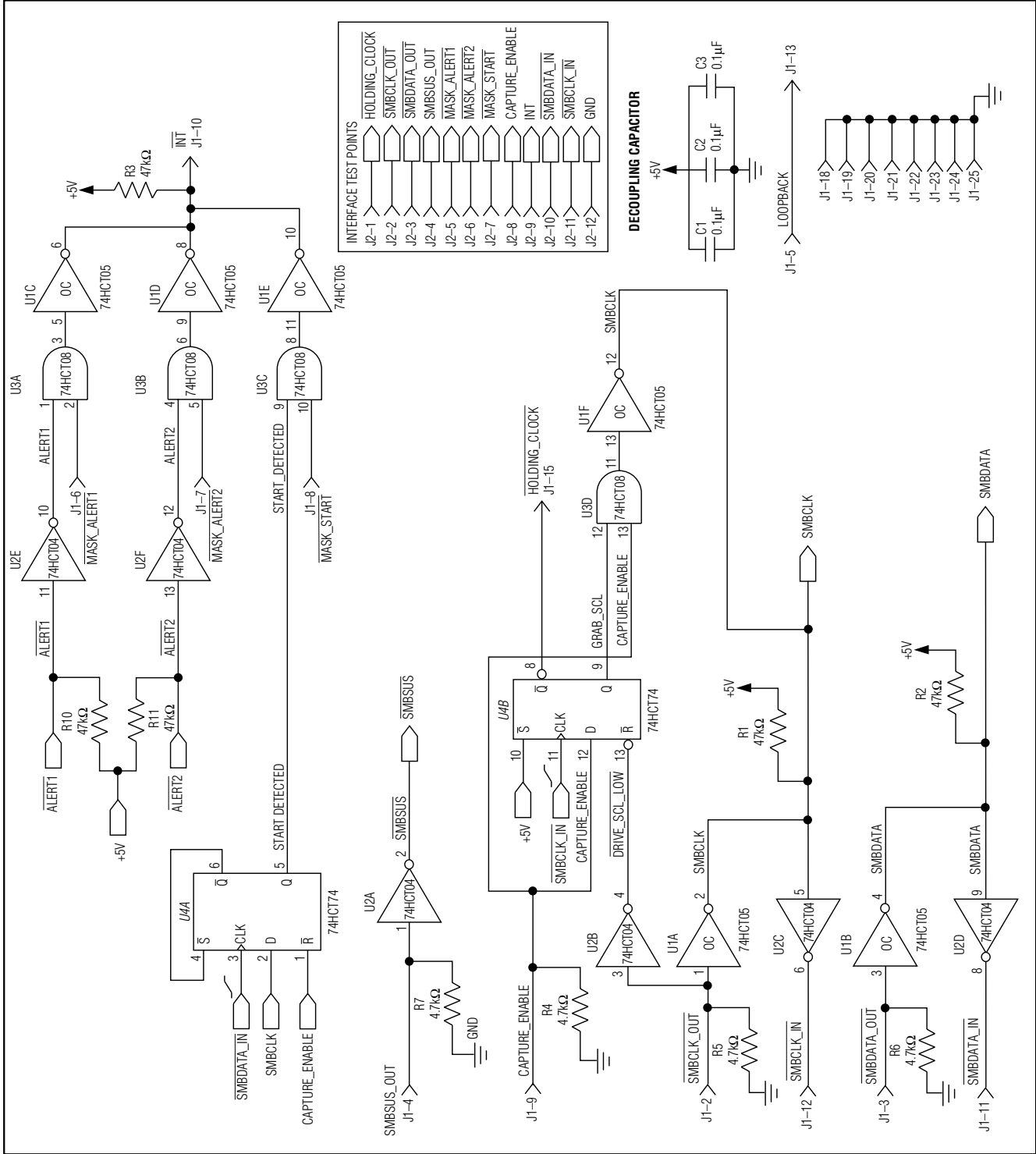
Figure 1a. MAXSMBus Schematic
