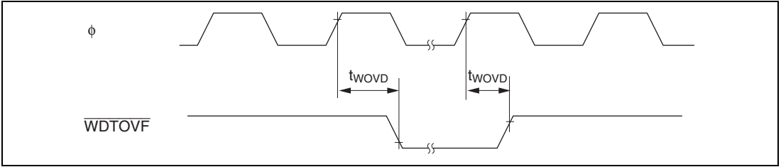
Figure 27.16 WDT0 Output Timing
