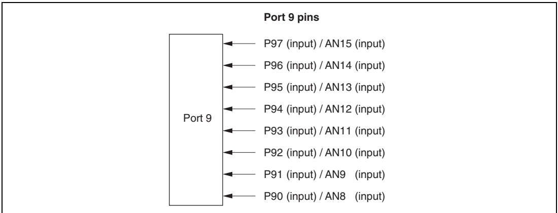
Figure 10B.5 Port 9 Pin Functions
