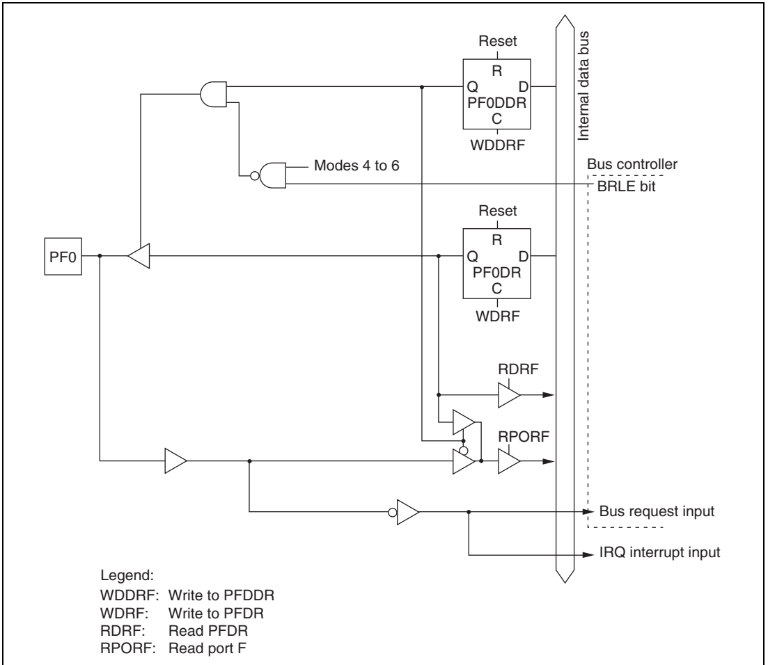
Figure C.23 (a) Port F Block Diagram (Pin PF0)
