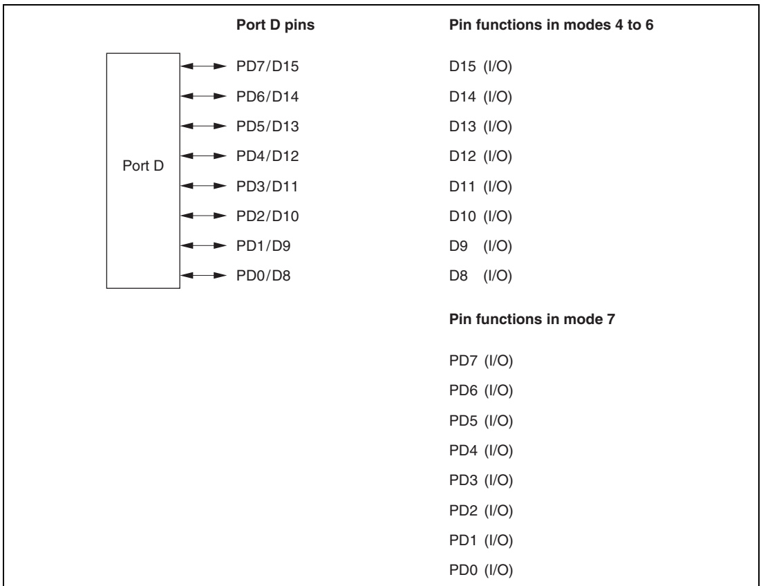
Figure 10A.12 Port D Pin Functions
