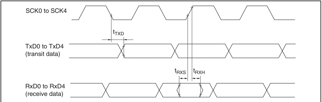
Figure 26.31 SCI Input/Output Timing (Clock Synchronous Mode)
