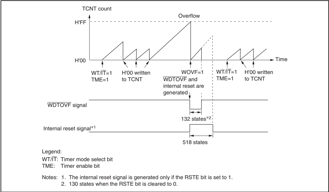
Figure 15.4 (a) WDT0 Watchdog Timer Operation
