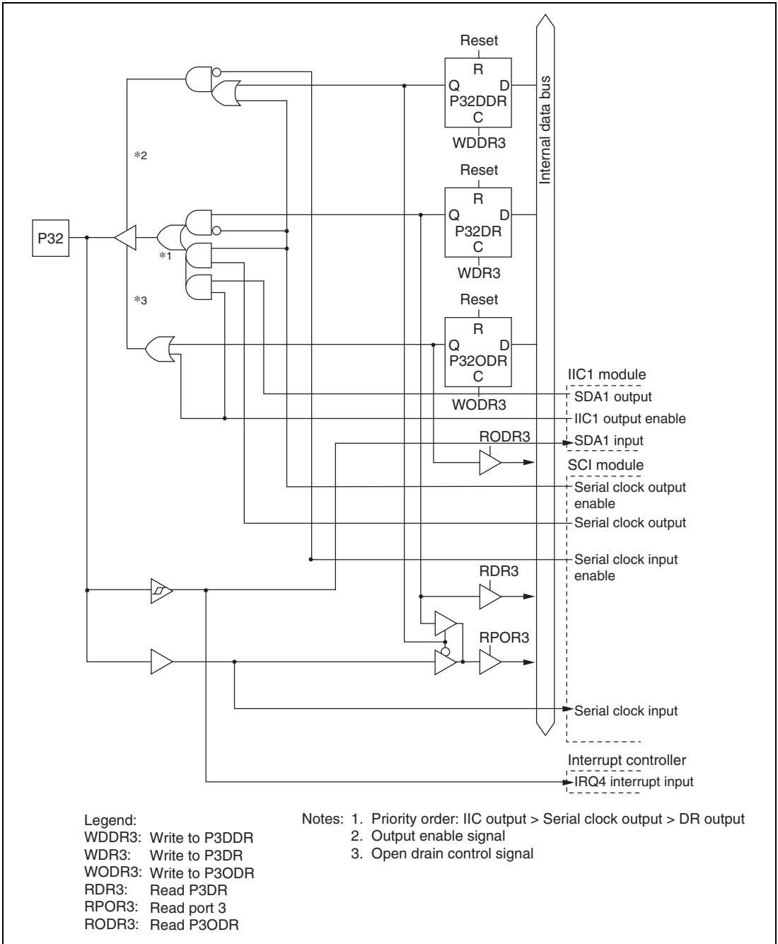
Figure C.2 (c) Port 3 Block Diagram (Pin P32)
