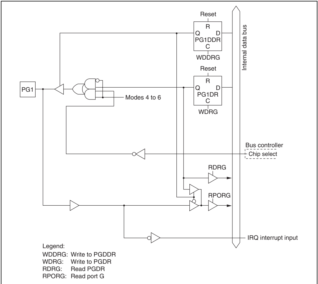
Figure C.24 (b) Port G Block Diagram (Pin PG1)
