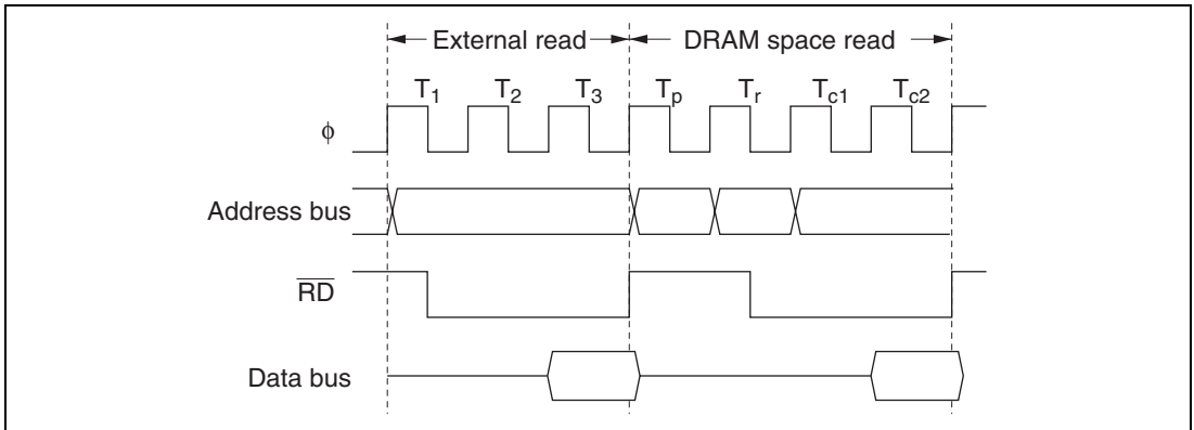
Figure 7.36 Example of DRAM Access after External Read
