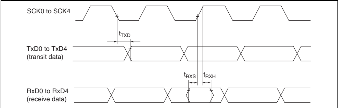
Figure 25.31 SCI Input/Output Timing (Clock Synchronous Mode)
