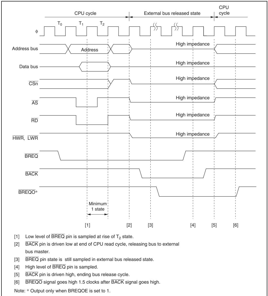
Figure 7.39 Bus-Released State Transition Timing
