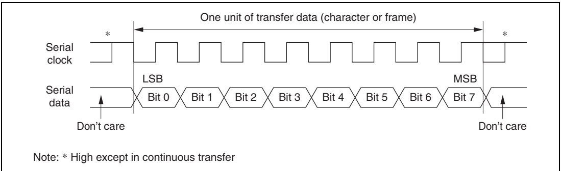
Figure 16.14 Data Format in Synchronous Communication
