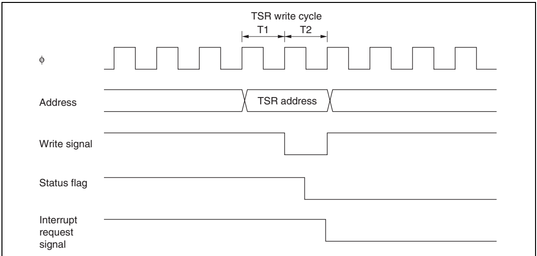
Figure 11.46 Timing for Status Flag Clearing by CPU
