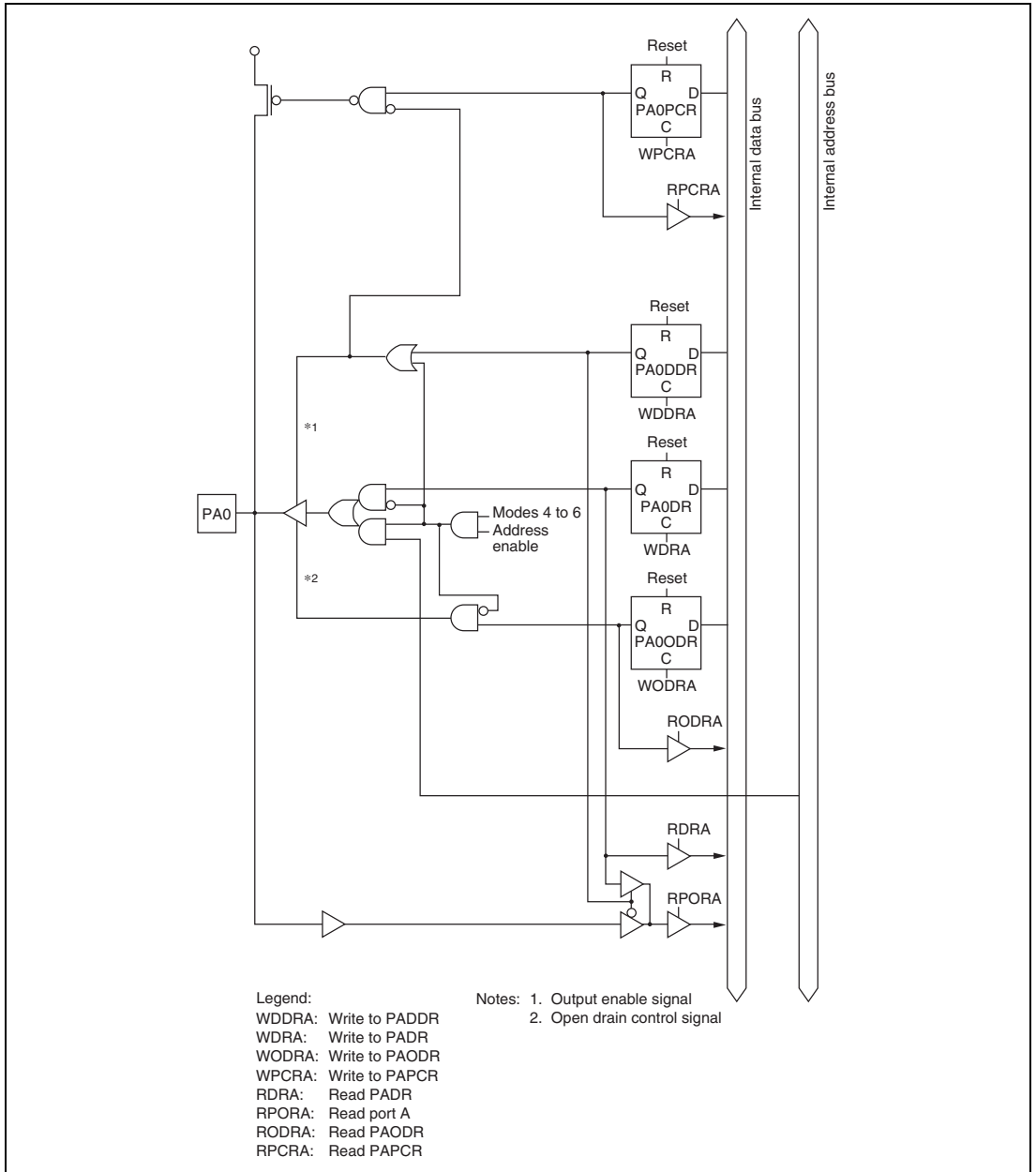
Figure C.18 (a) Port A Block Diagram (Pin PA0)
