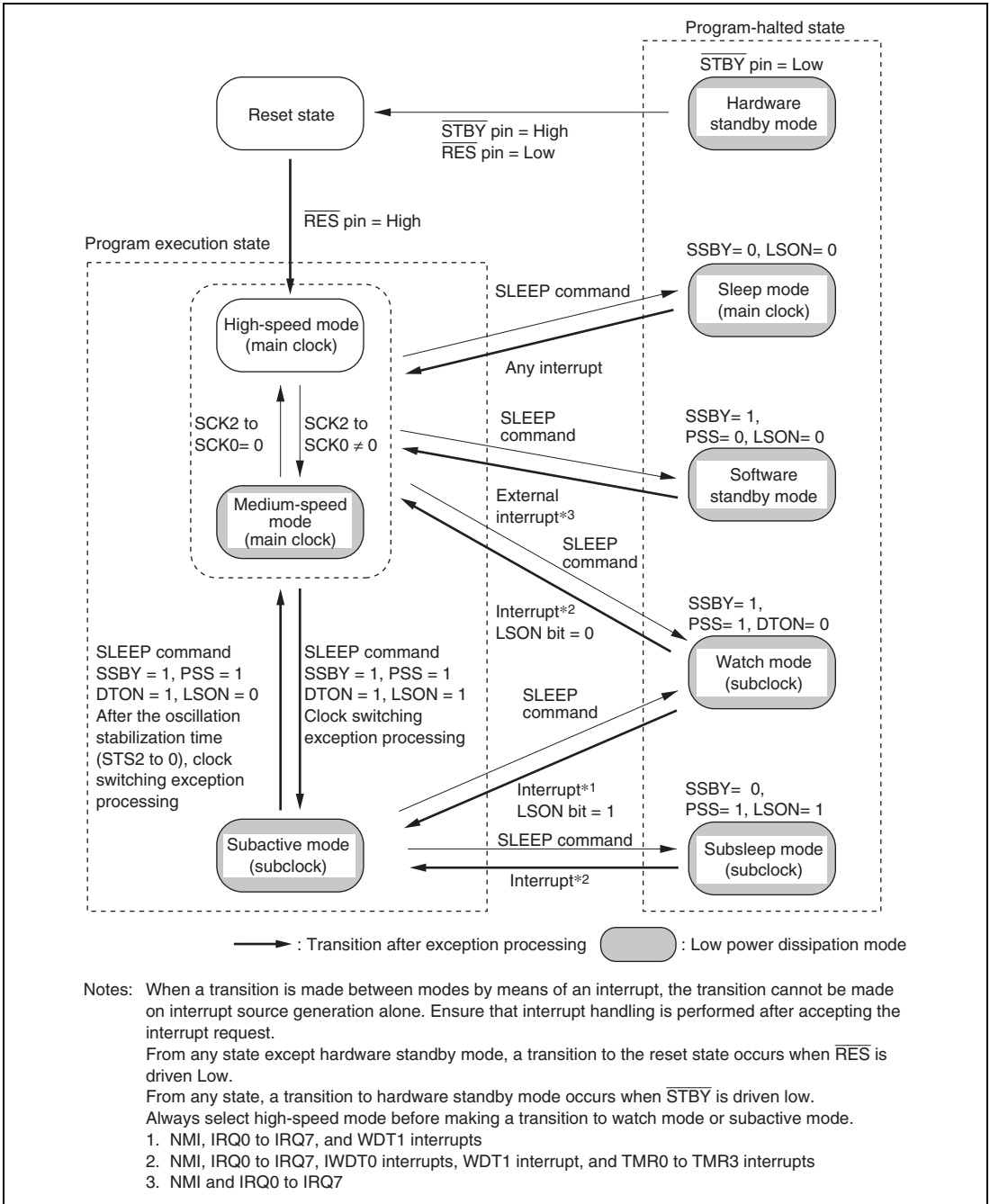
Figure 24.1 (a) Mode Transition Diagram (H8S/2633 Group, H8S/2633R)
