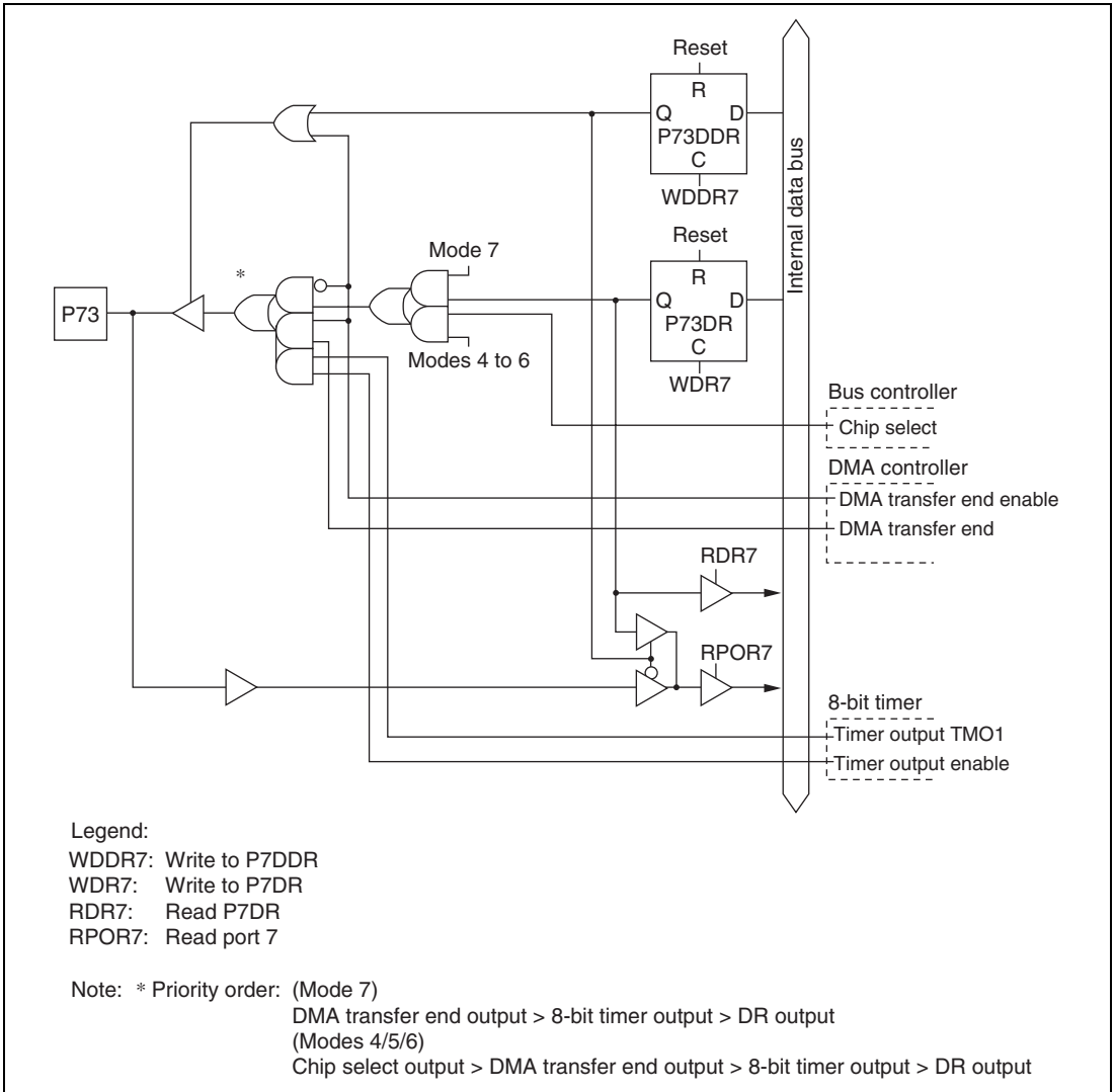
Figure C.4 (c) Port 7 Block Diagram (Pin P73)
