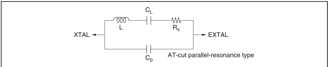
Figure 23A.3 Crystal Resonator Equivalent Circuit
