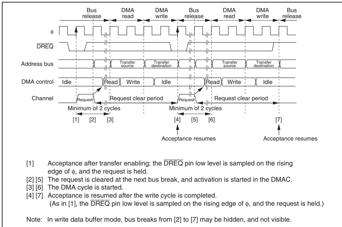
Figure 8.25 Example of DREQ Level Activated Normal Mode Transfer
