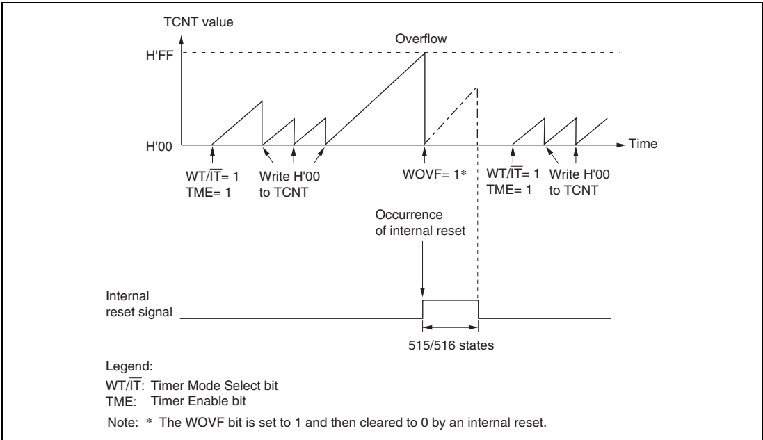
Figure 15.4 (b) WDT1 Operation in Watchdog Timer Mode
