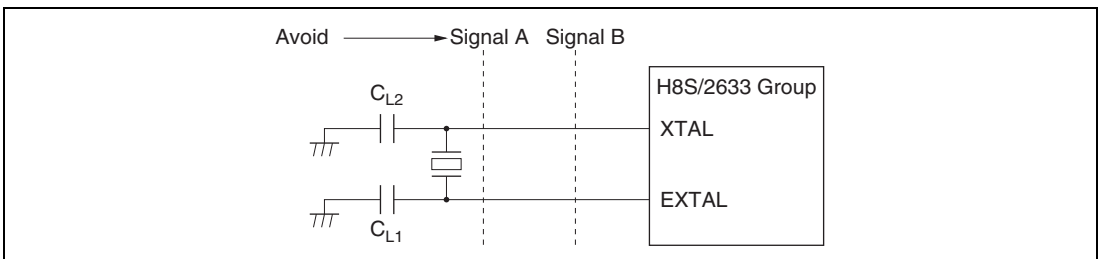
Figure 23A.4 Example of Incorrect Board Design
