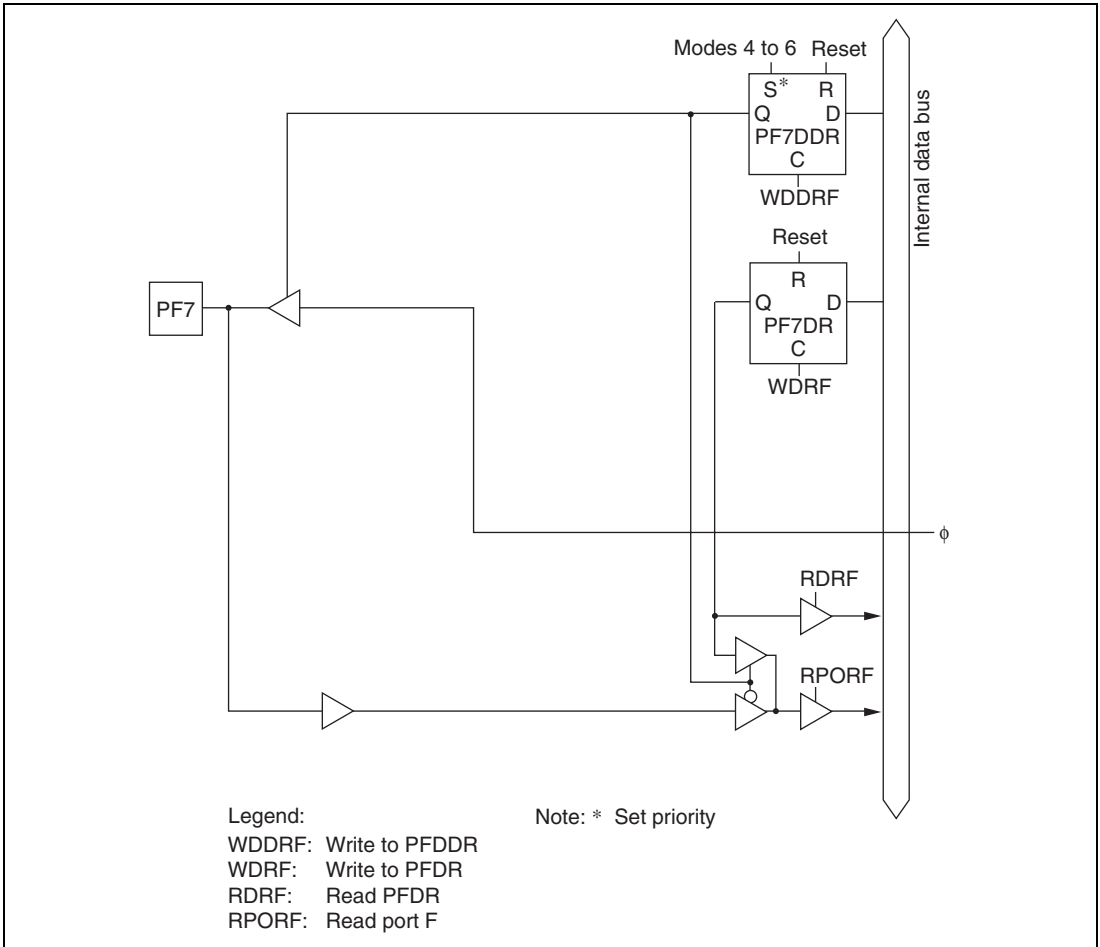
Figure C.23 (h) Port F Block Diagram (Pin PF7)
