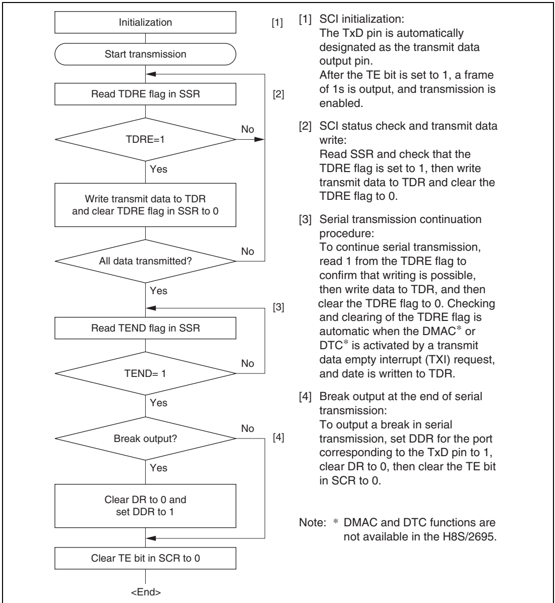
Figure 16.5 Sample Serial Transmission Flowchart
