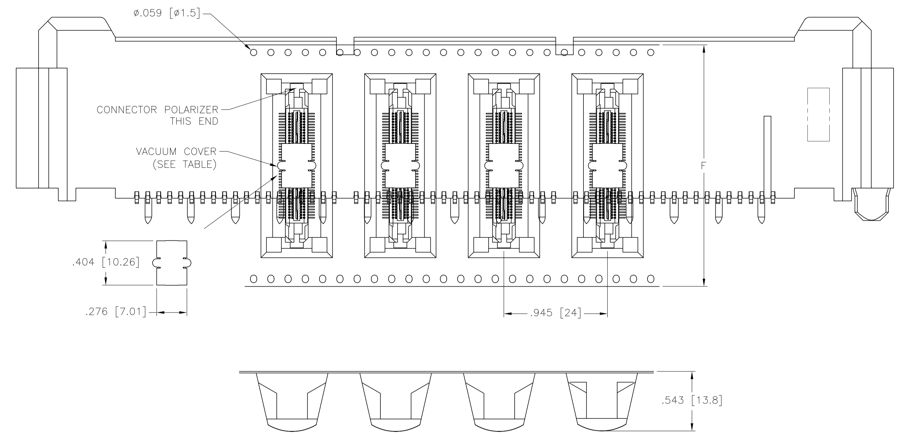
PACKAGING DETAIL \triangle 7 SCALE 2:1 DIMENSIONS ARE FOR REFERENCE
