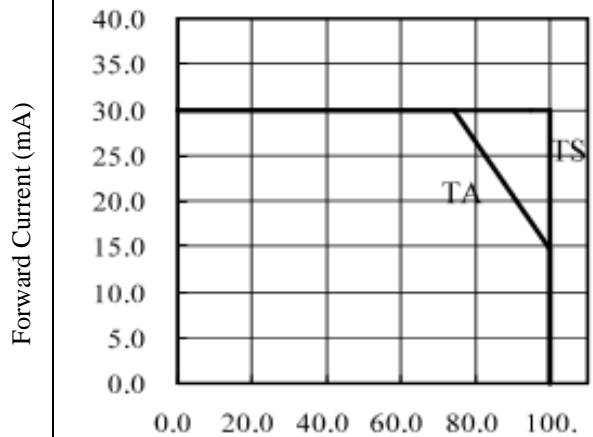
Max. Permissible Forward Current ( T_a=25^\circ\text{C} )
