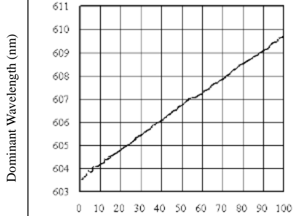
Dominant Wavelength vs. Forward Current ( T_a=25^\circ\text{C} )
