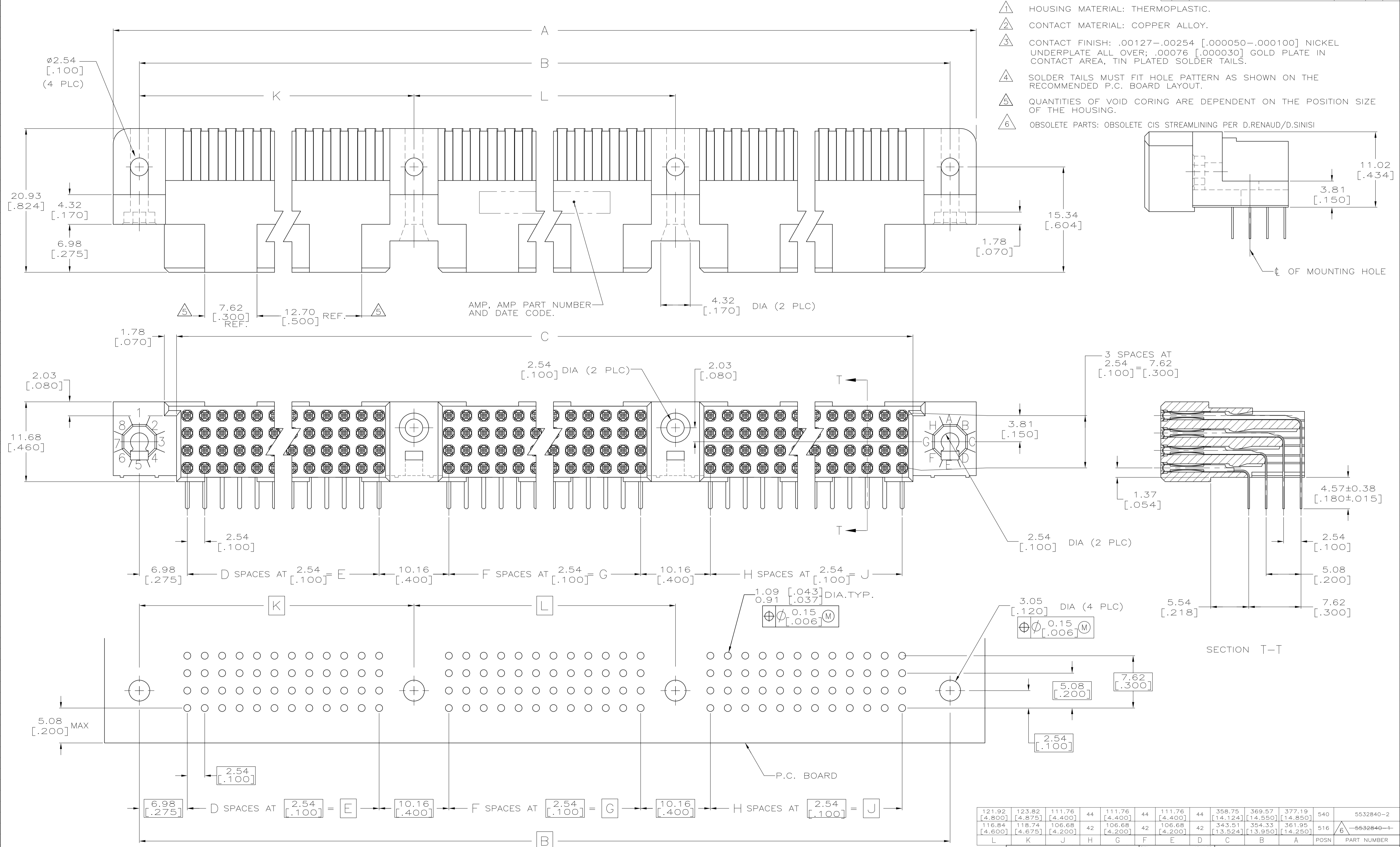
RECOMMENDED P.C. BOARD LAYOUT 4
