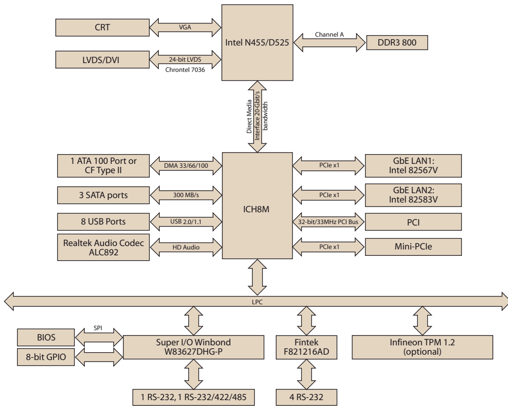
Figure 1.3 AIMB-213 Board Diagram
