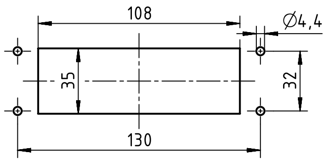
Panel cut out (1:2)
