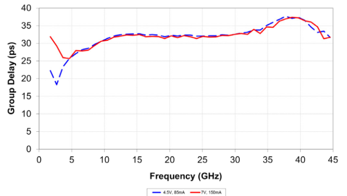
Typical IC performance measured on-wafer
