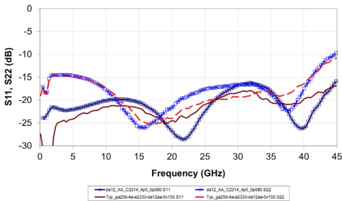
Typical IC performance measured on-wafer
