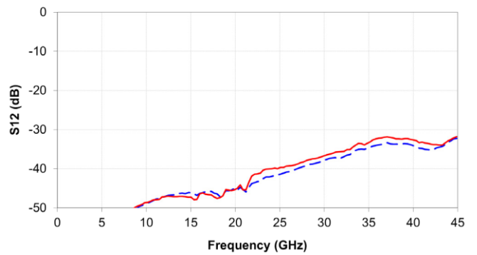
Typical IC performance measured on-wafer
