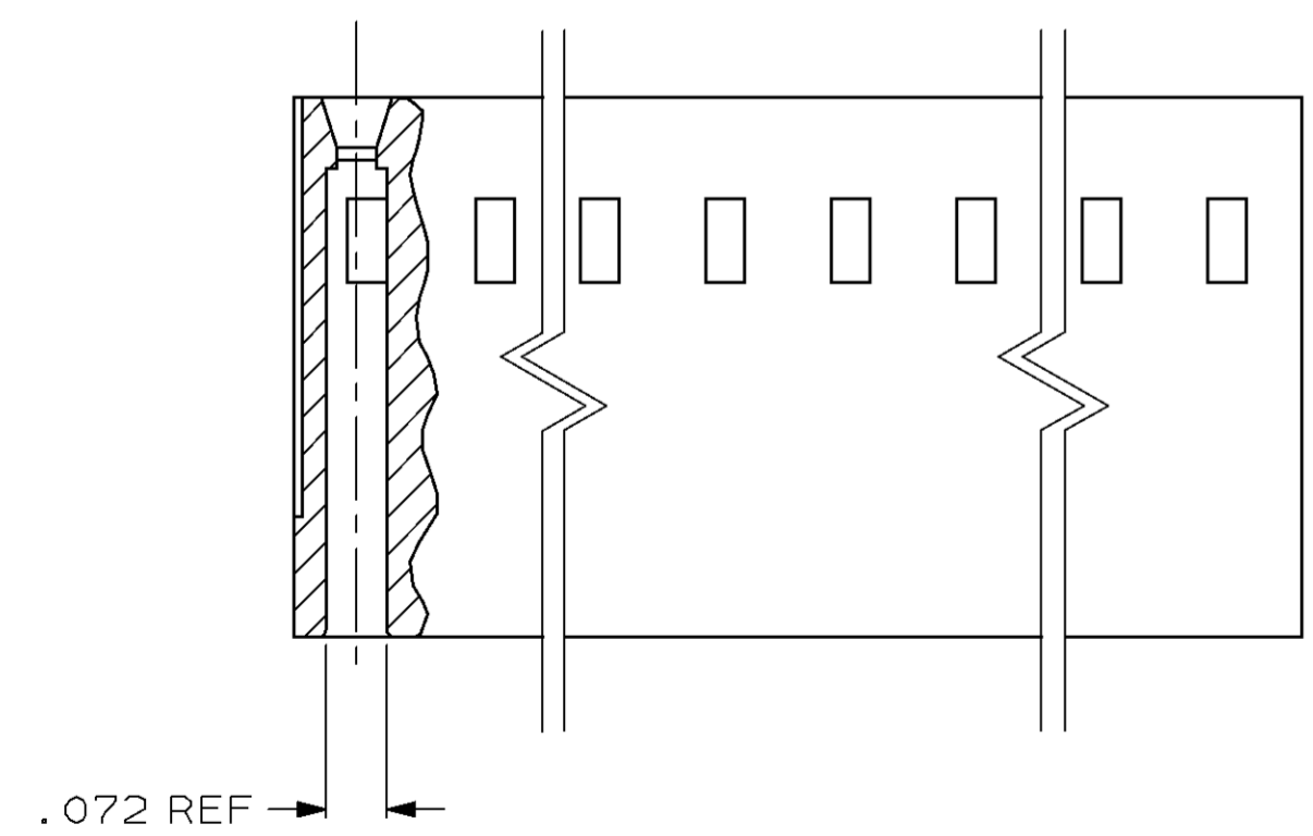
SECT X-X
