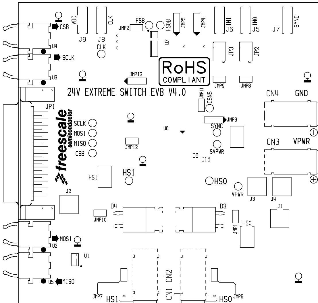
Figure 10. KIT10XS4200EVBE Silkscreen
