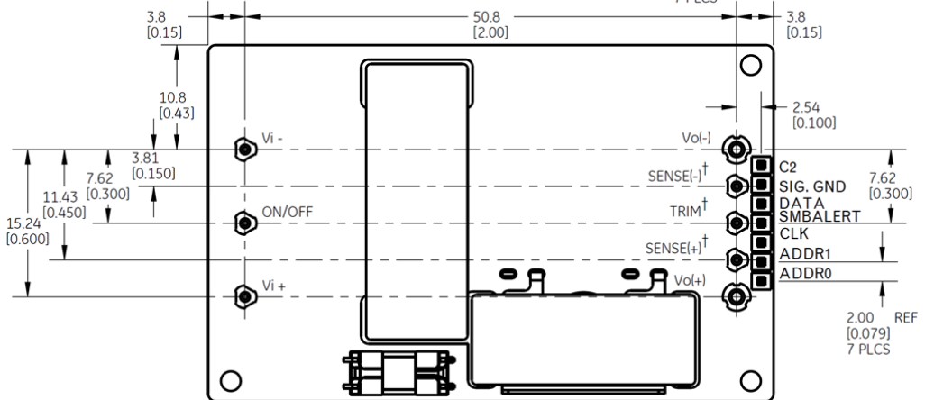
BOTTOM VIEW
