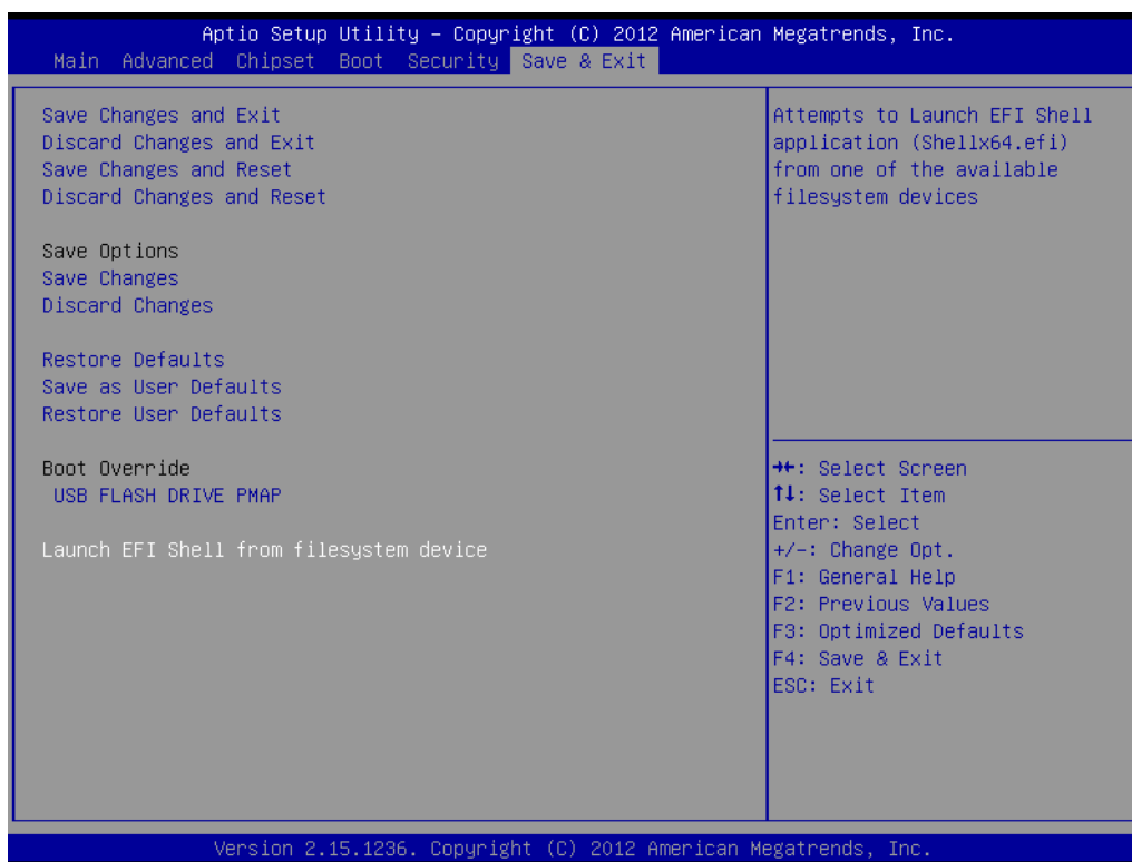
Figure 3.29 Save & Exit
