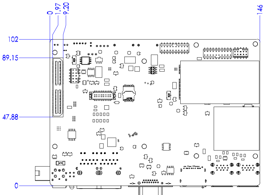
Figure 1.2 MIO-5271 Mechanical Drawing (Bottom Side)
